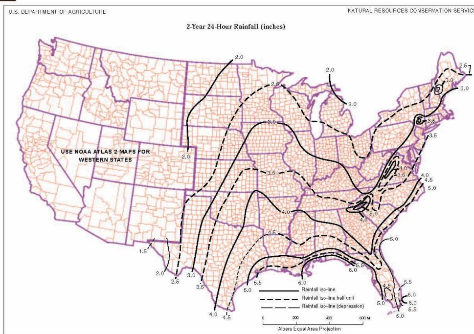
Figure B-3 2-year, 24-hr rainfall
