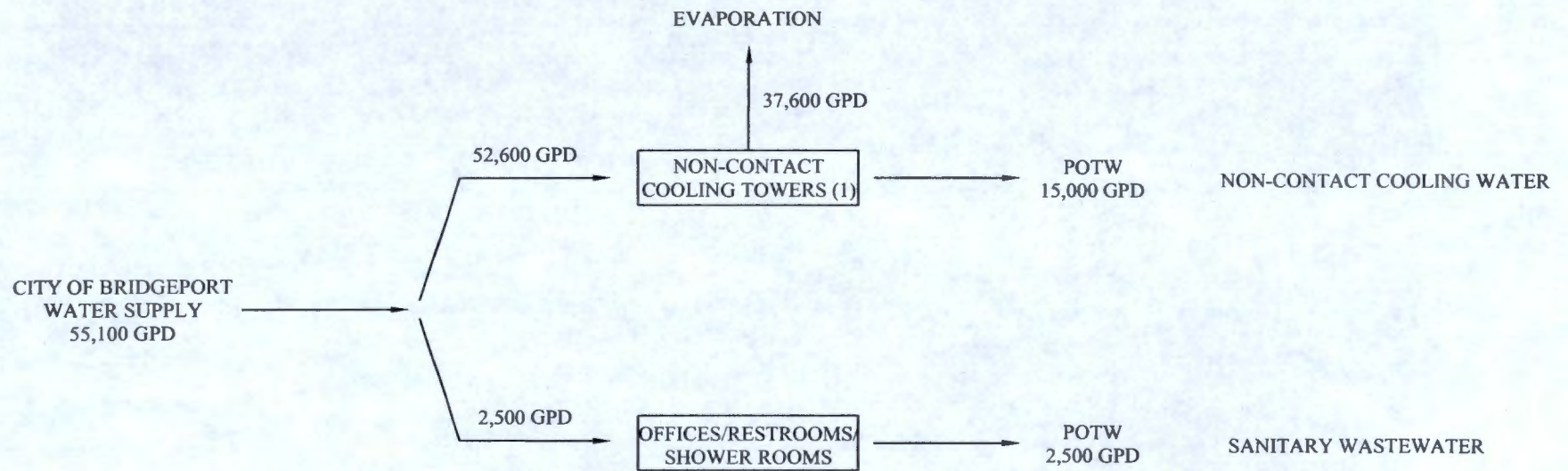
FIGURE 3 FERROGLOBE USA BRIDGEPORT WATER FLOW SCHEMATIC
