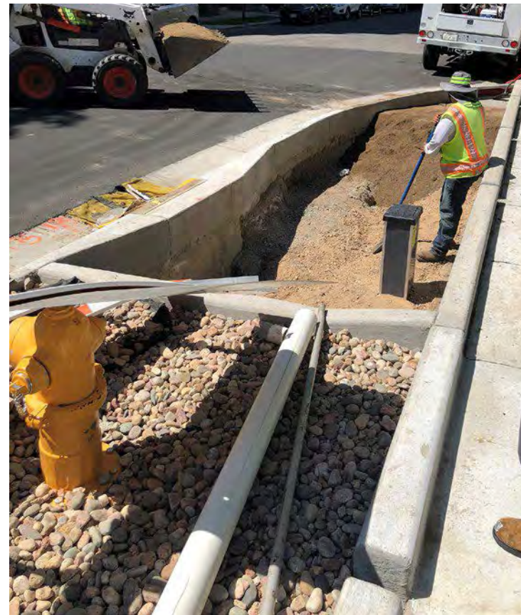
Installing BSM amended with biochar, zeolite, and coconut coir in Denver, CO.
