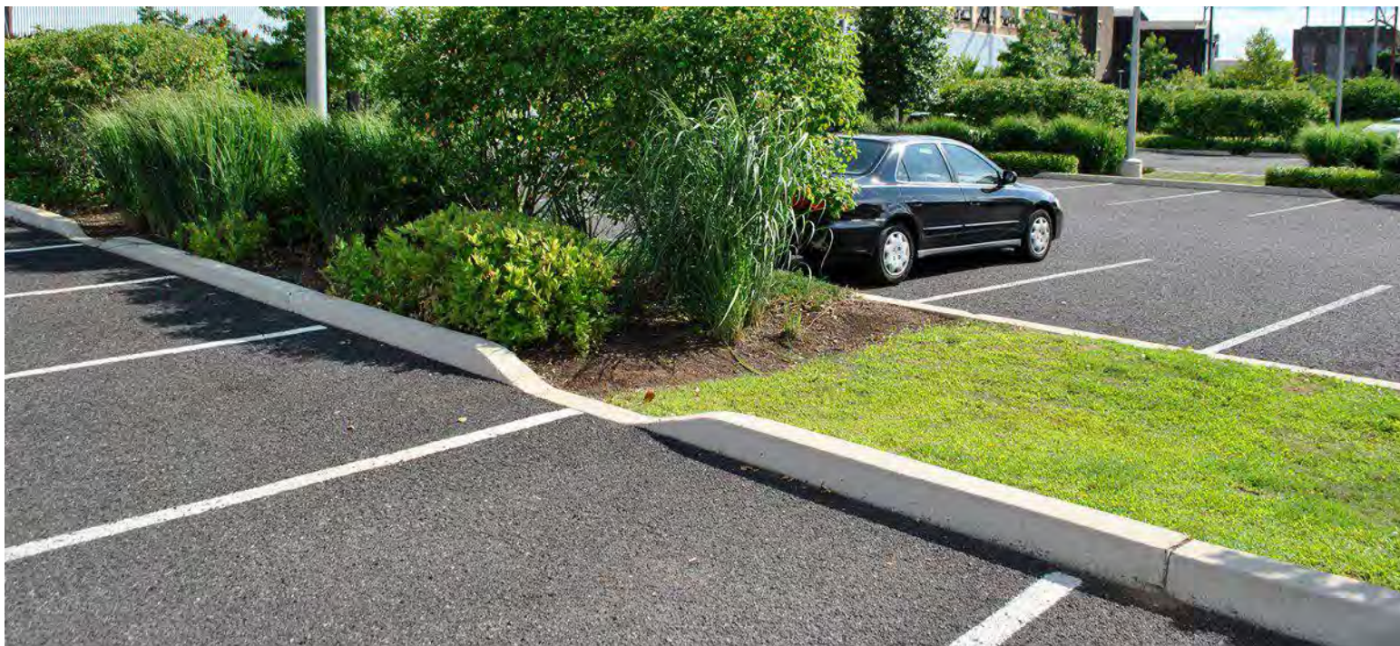
A bioretention practice in Philadelphia, PA, with a wide curb opening and angled edges to facilitate runoff capture.
