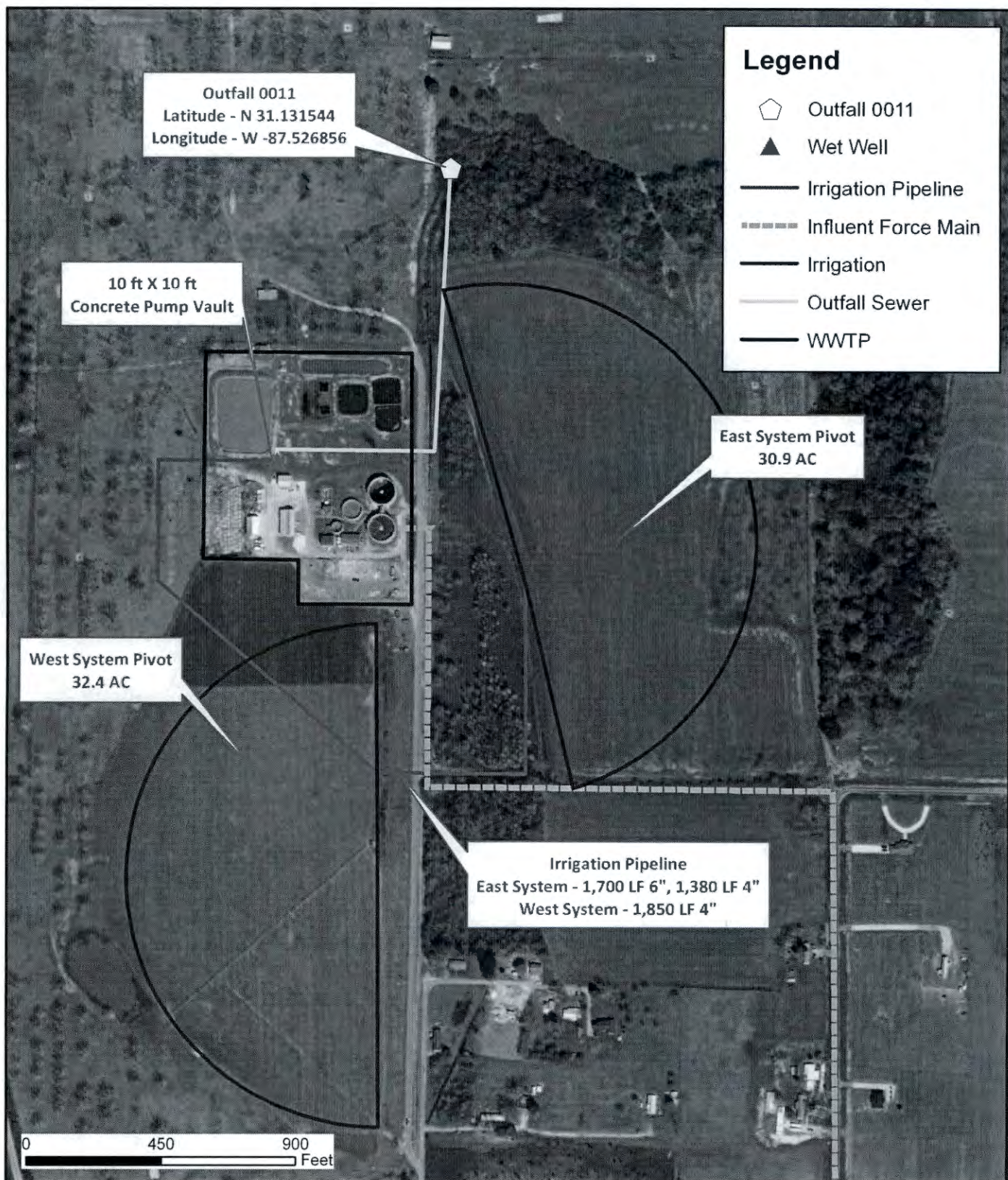
Figure 2 WWTP System Overview
