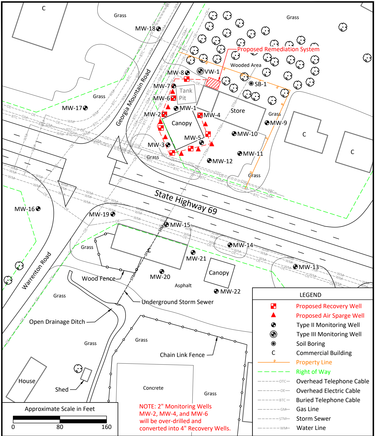
Proposed System Layout Map
