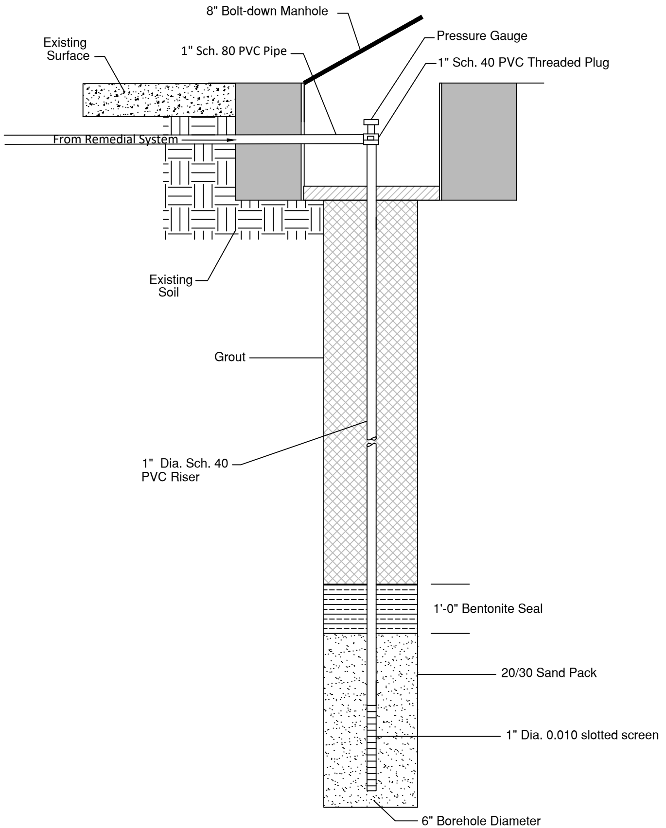
Air Sparge Well Construction Detail
