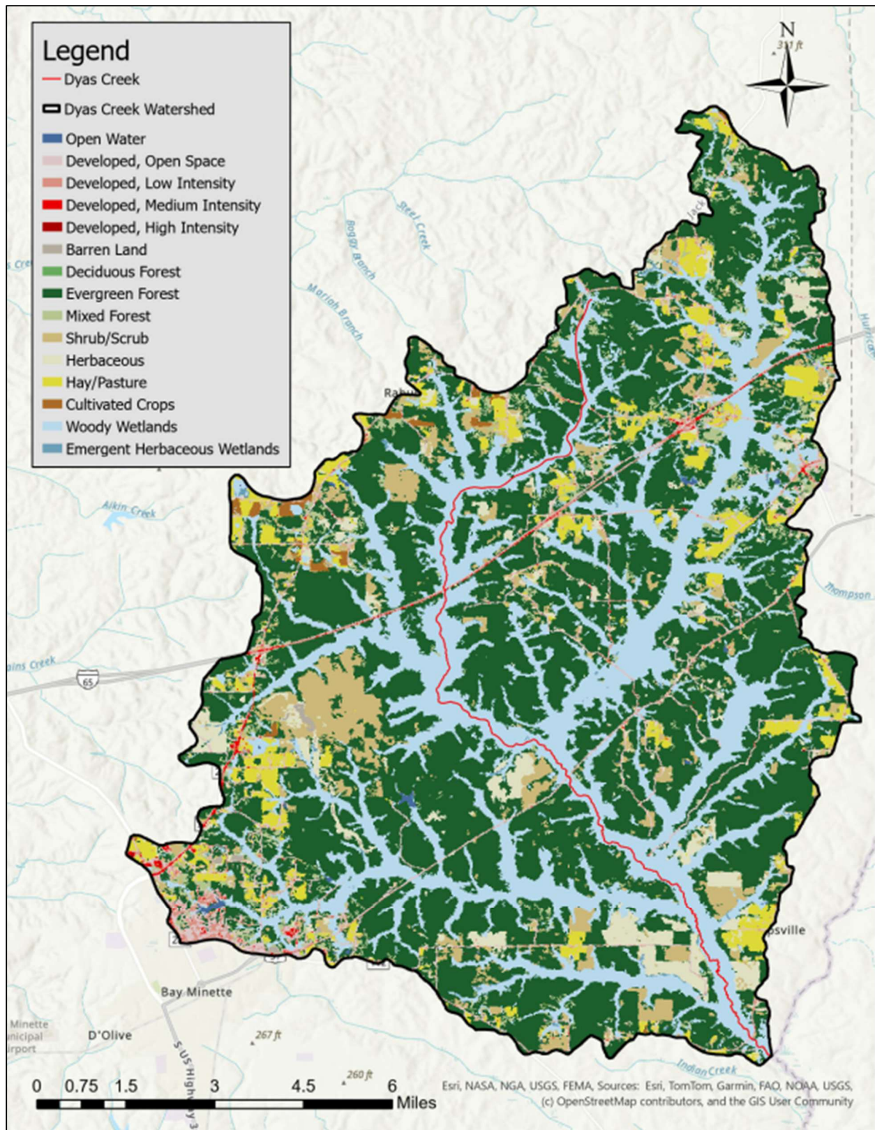
Figure 3: 2021 NLCD Map of the Dyas Creek Watershed
