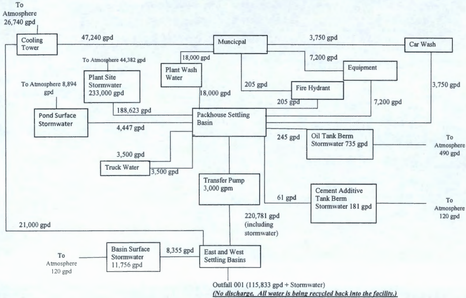
Schematic of Water Flow
