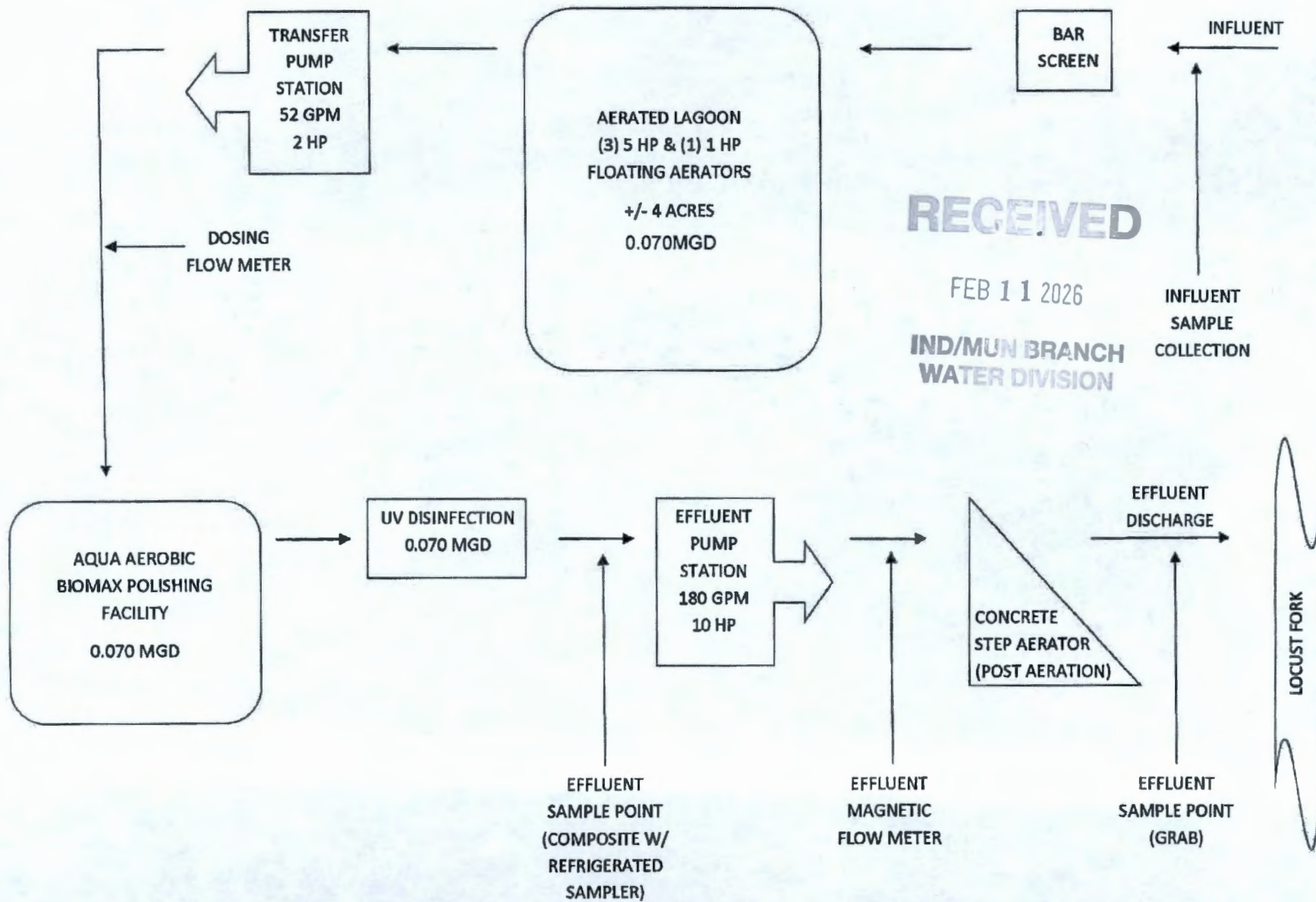
ALTOONA LAGOON FLOW SCHEMATIC
