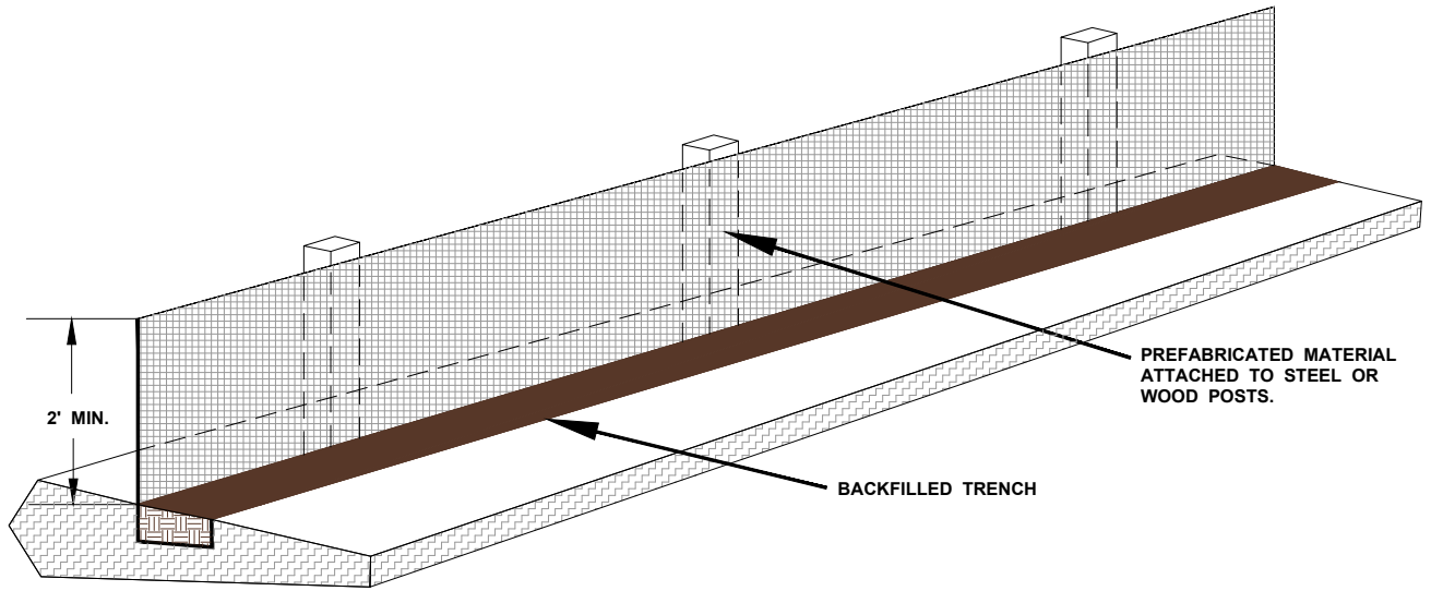
PREFABRICATED FILTER FENCE DETAIL
