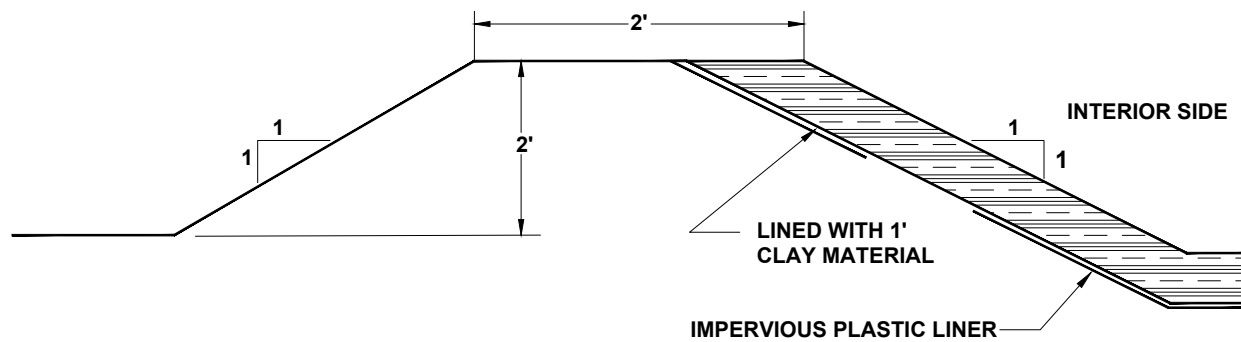
SIDE VIEW
