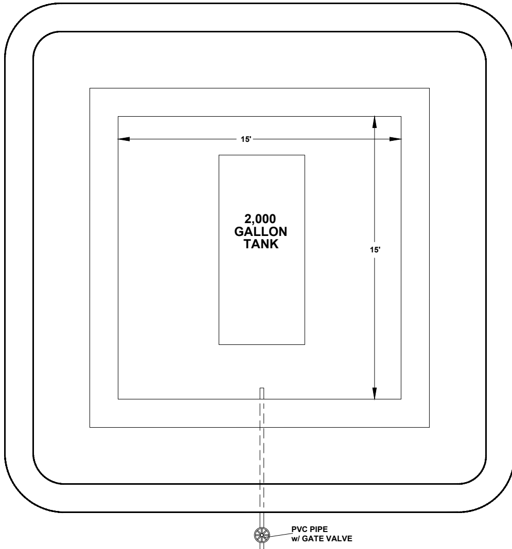
PLAN VIEW
