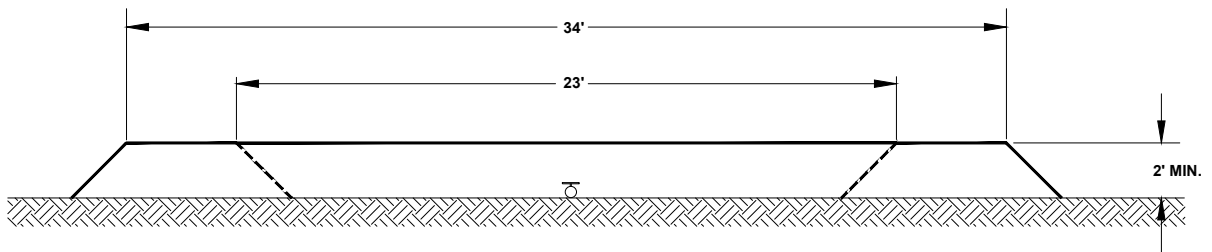
ELEVATION VIEW
