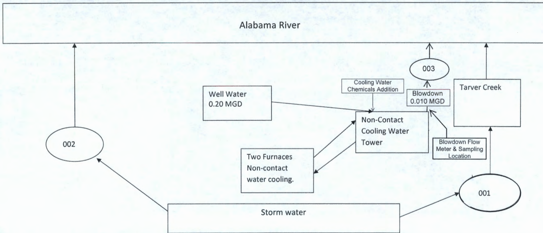
Figure 3 Ferroglobe USA Metallurgical Inc. – Selma Plant Water Flow Schematic April 2025
