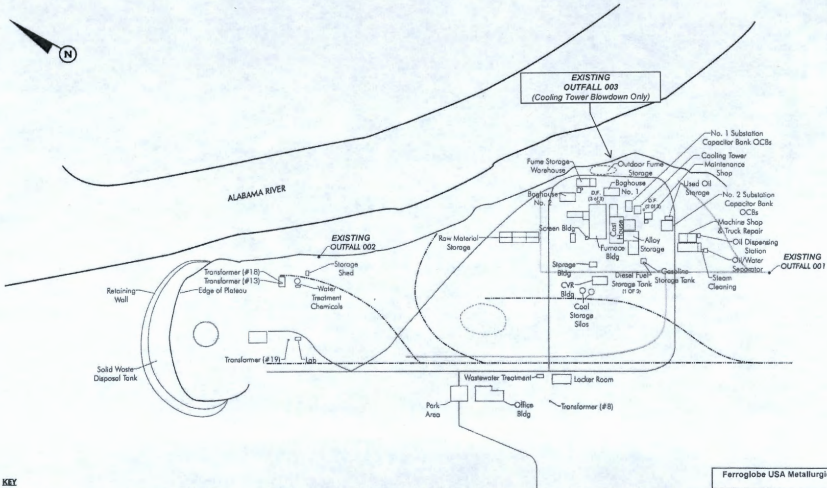
Figure 2 Site Plan
