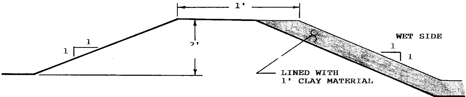
SIDE VIEW
