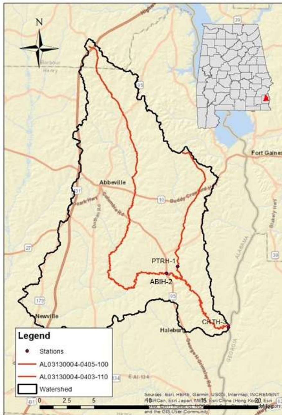
Figure 3.5.1: ADEM sampling stations in the Abbie Creek watershed
