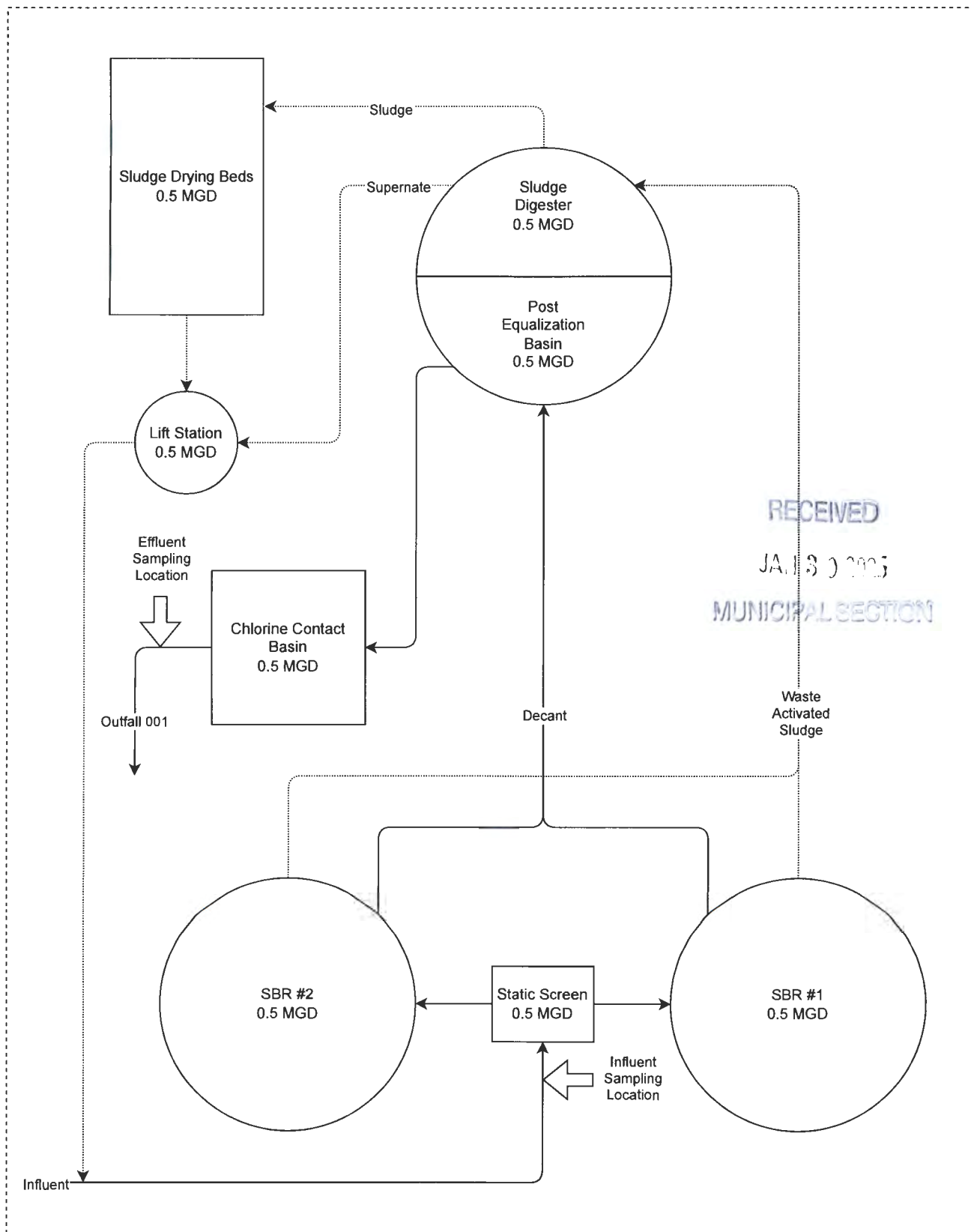
Cordova WWTP Flow Schematic
