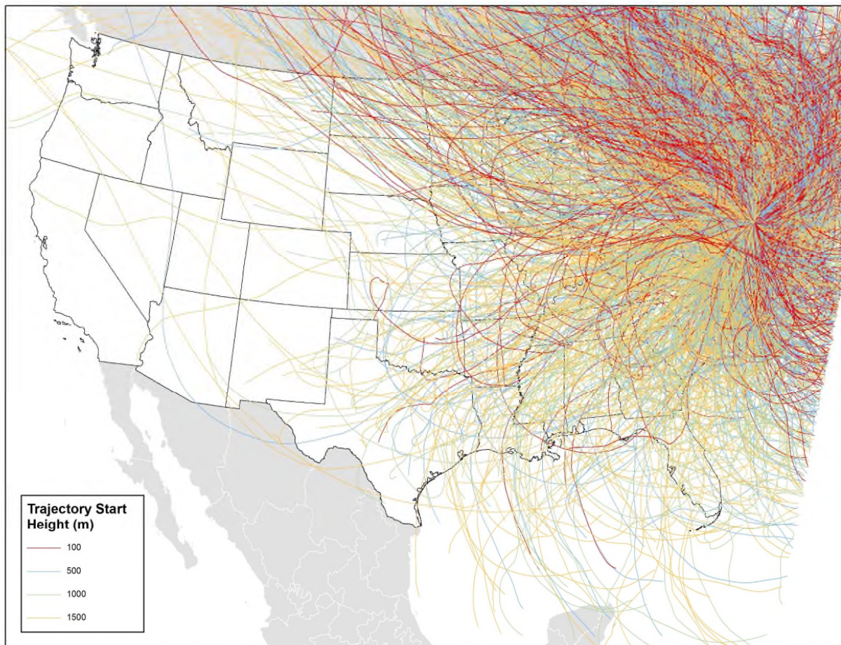
Figure 3: 100-Meter, 500-Meter, 1000-Meter, and 1500-Meter Back Trajectories for the 20% Most Impaired Days (2011-2016) from Brigantine Wilderness Area
