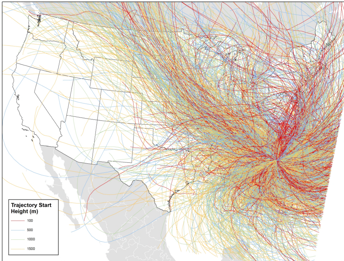
Figure 3: 100-Meter, 500-Meter, 1000-Meter, and 1500-Meter Back Trajectories for the 20% Most Impaired Days (2011-2016) from Wolf Island Wilderness Area
