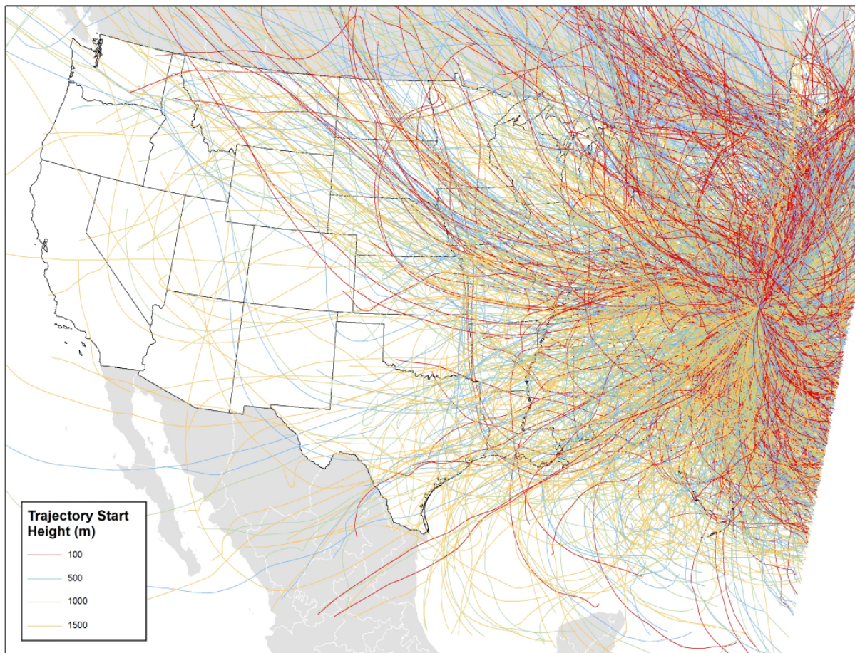
Figure 3: 100-Meter, 500-Meter, 1000-Meter, and 1500-Meter Back Trajectories for the 20% Most Impaired Days (2011-2016) from Swanquarter Wilderness Area
