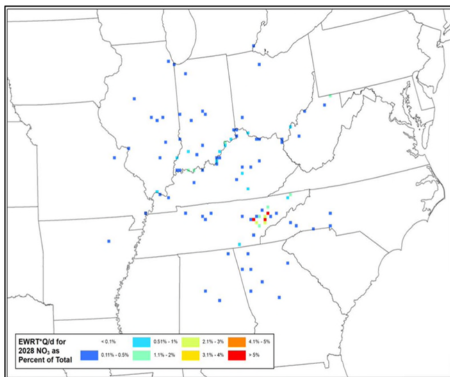
Figure 9: Nitrate Emissions/Distance Extinction Weighted Residence Time (% of Total Q/d*EWRT per 12km Modeling Grid Cell) for Great Smoky Mountains National Park – Full View (top) and Class I Zoom (bottom)
