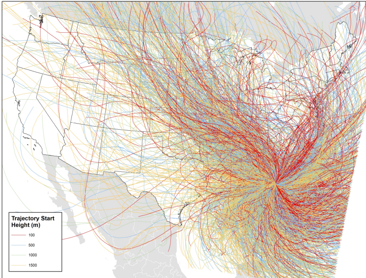
Figure 3: 100-Meter, 500-Meter, 1000-Meter, and 1500-Meter Back Trajectories for the 20% Most Impaired Days (2011-2016) from St Marks Wilderness Area
