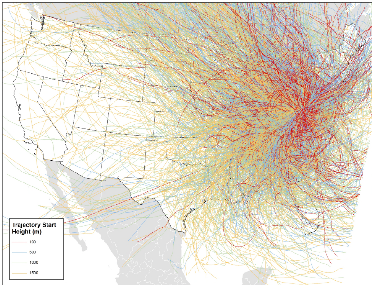
Figure 3: 100-Meter, 500-Meter, 1000-Meter, and 1500-Meter Back Trajectories for the 20% Most Impaired Days (2011-2016) from Dolly Sods Wilderness Area
