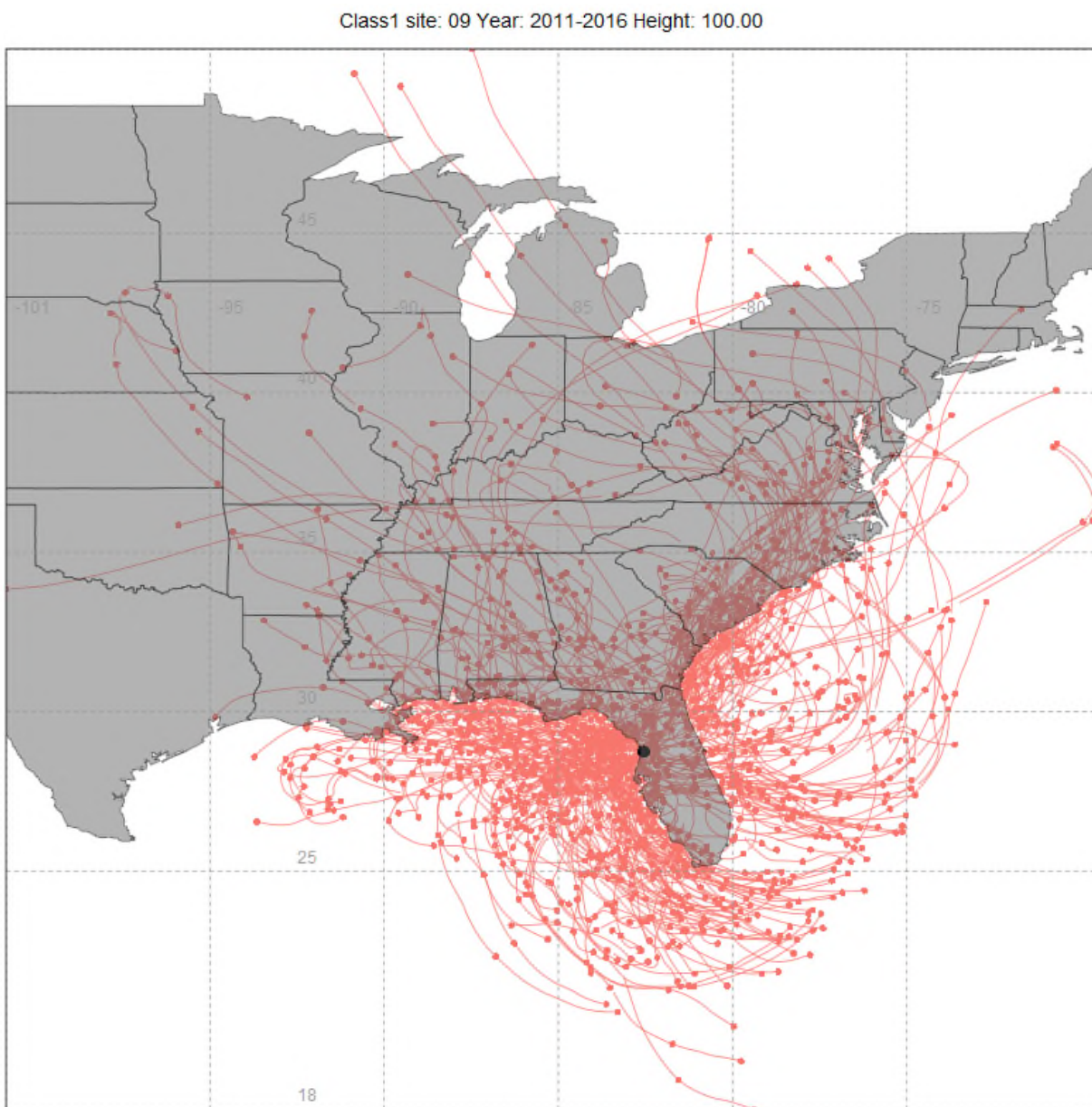
Figure 1: 100-Meter Back Trajectories for the 20% Most Impaired Visibility Days (2011-2016), from Chassahowitzka Wilderness Area
