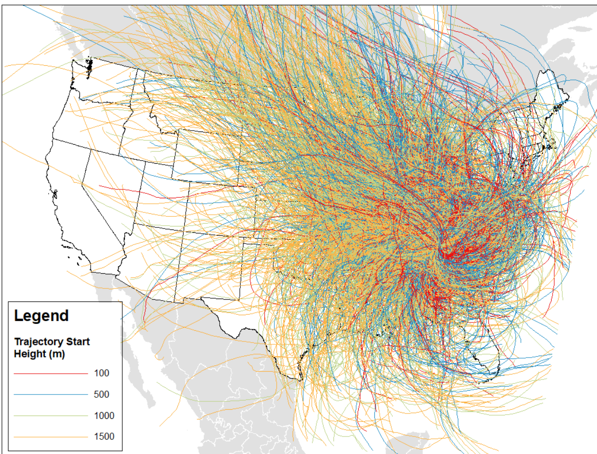
Figure 3: 100-Meter, 500-Meter, 1000-Meter, and 1500-Meter Back Trajectories for the 20% Most Impaired Days (2011-2016) from Great Smoky Mountains National Park
