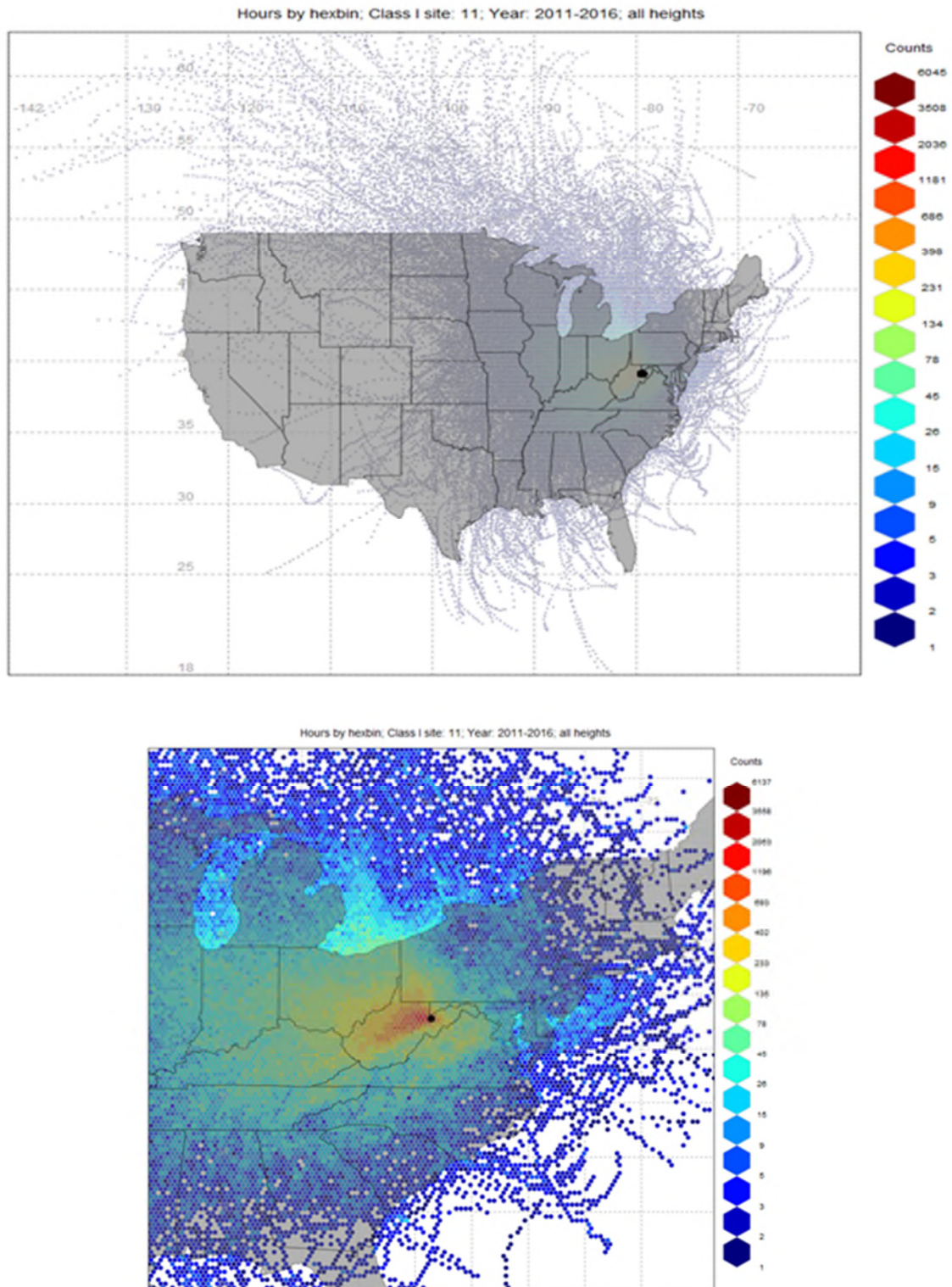
Figure 4: Residence Time (Counts per 12km Modeling Grid Cell) for Dolly Sods Wilderness Area – Full View (top) and Class I Zoom (bottom)
