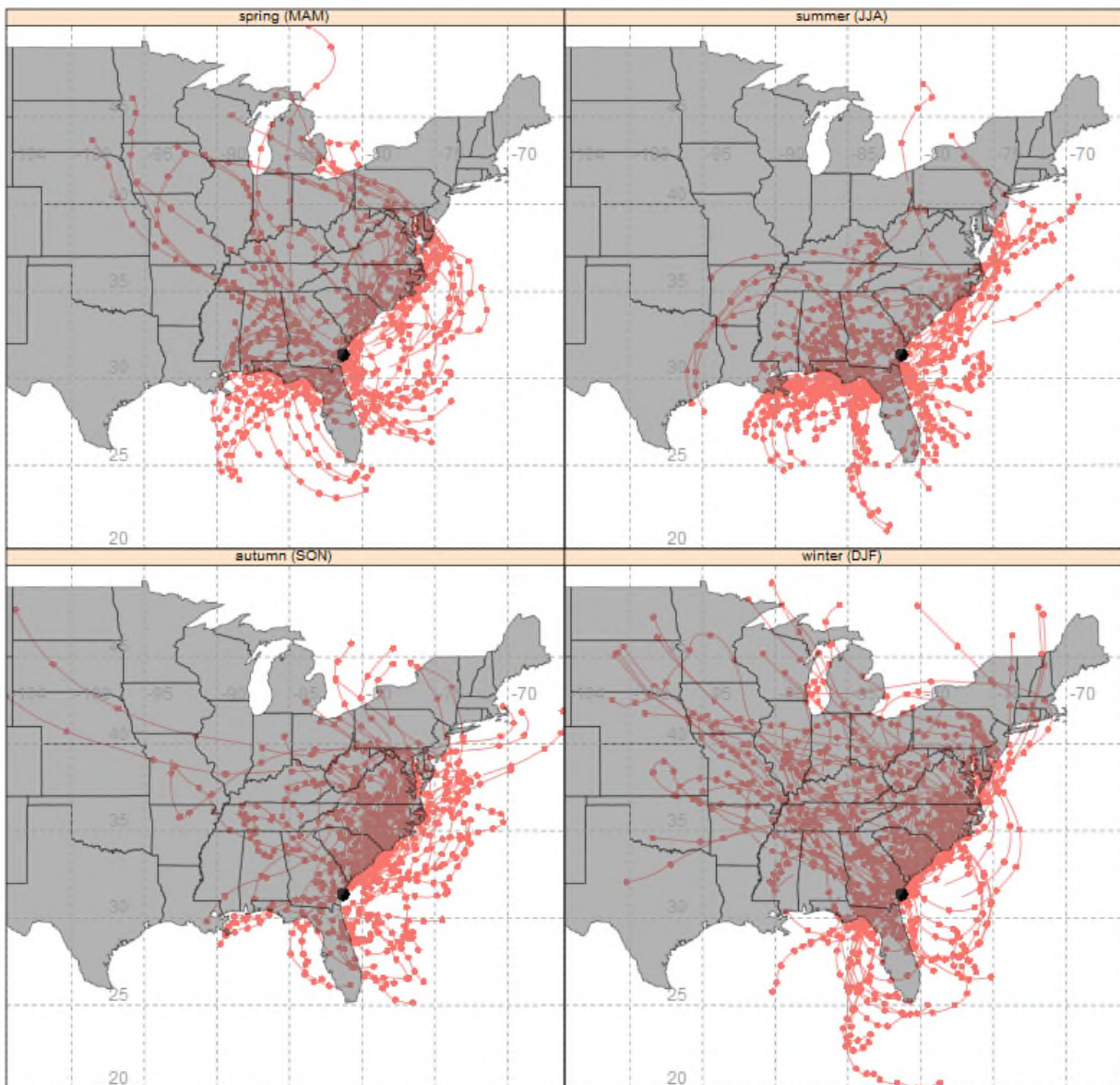
Figure 2: 100-Meter Back Trajectories by Season for the 20% Most Impaired Visibility Days (2011-2016) from Wolf Island Wilderness Area
