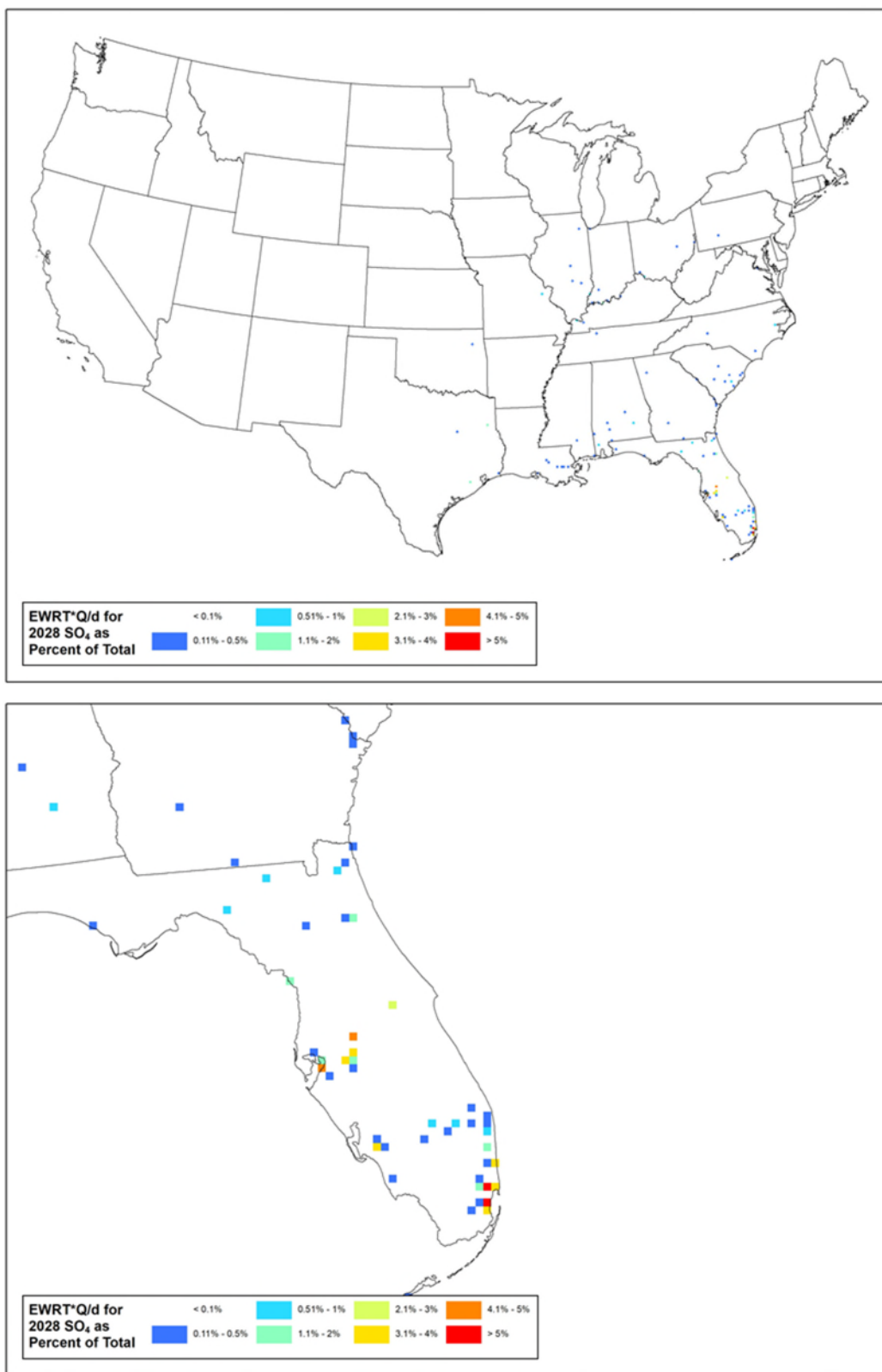
Figure 8: Sulfate Emissions/Distance Extinction Weighted Residence Time (% of Total Q/d \cdot EWRT per 12km Modeling Grid Cell) for Everglades National Park – Full View (top) and Class I Zoom (bottom)
