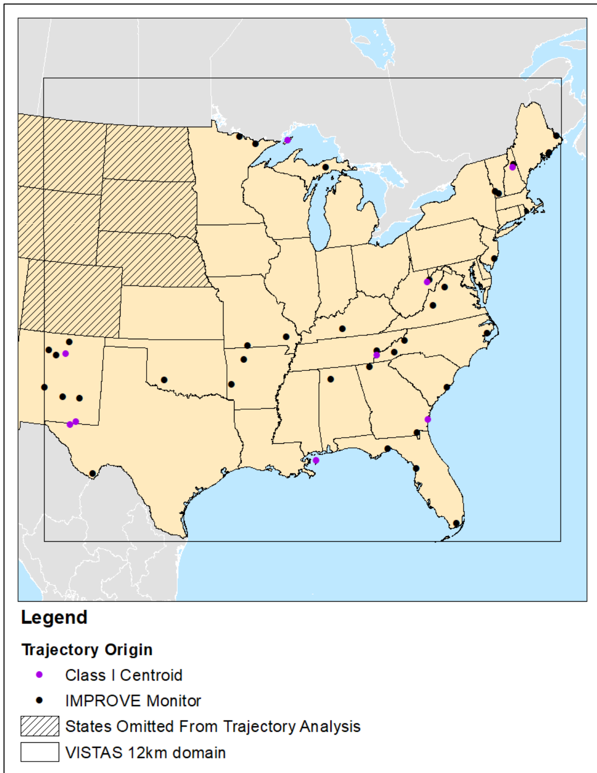
Figure 2-1. IMPROVE Monitor Locations and Starting Points for HYSPLIT Trajectories in the VISTAS 12km Domain
