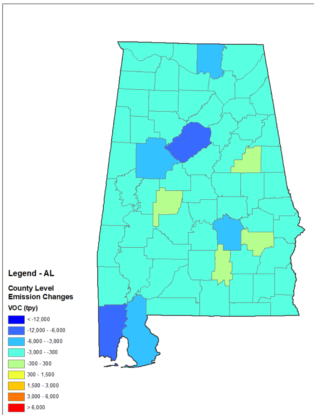
Figure E.1-7. Alabama County Level VOC Emissions Changes from the EPA 2011 Base Year Inventory to the Revised 2028 Inventory (except Biogenic)
