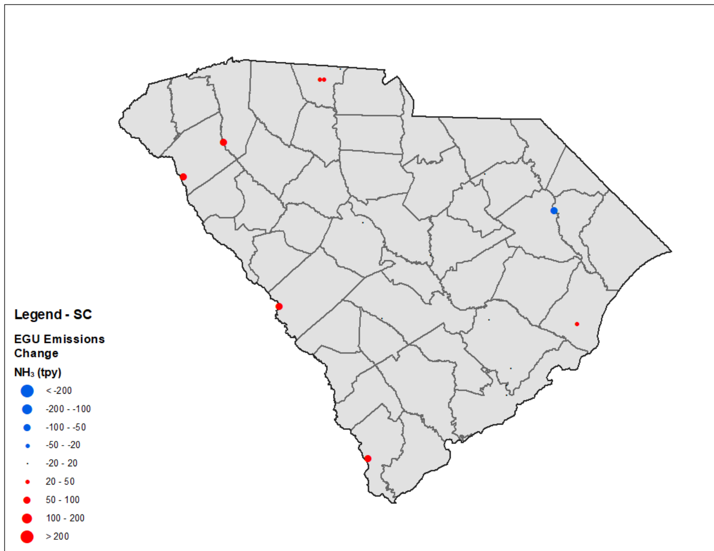
Figure C.7-3. South Carolina Point EGU NH 3 Emissions Changes from the EPA 2028el Inventory to the Revised 2028 Inventory
