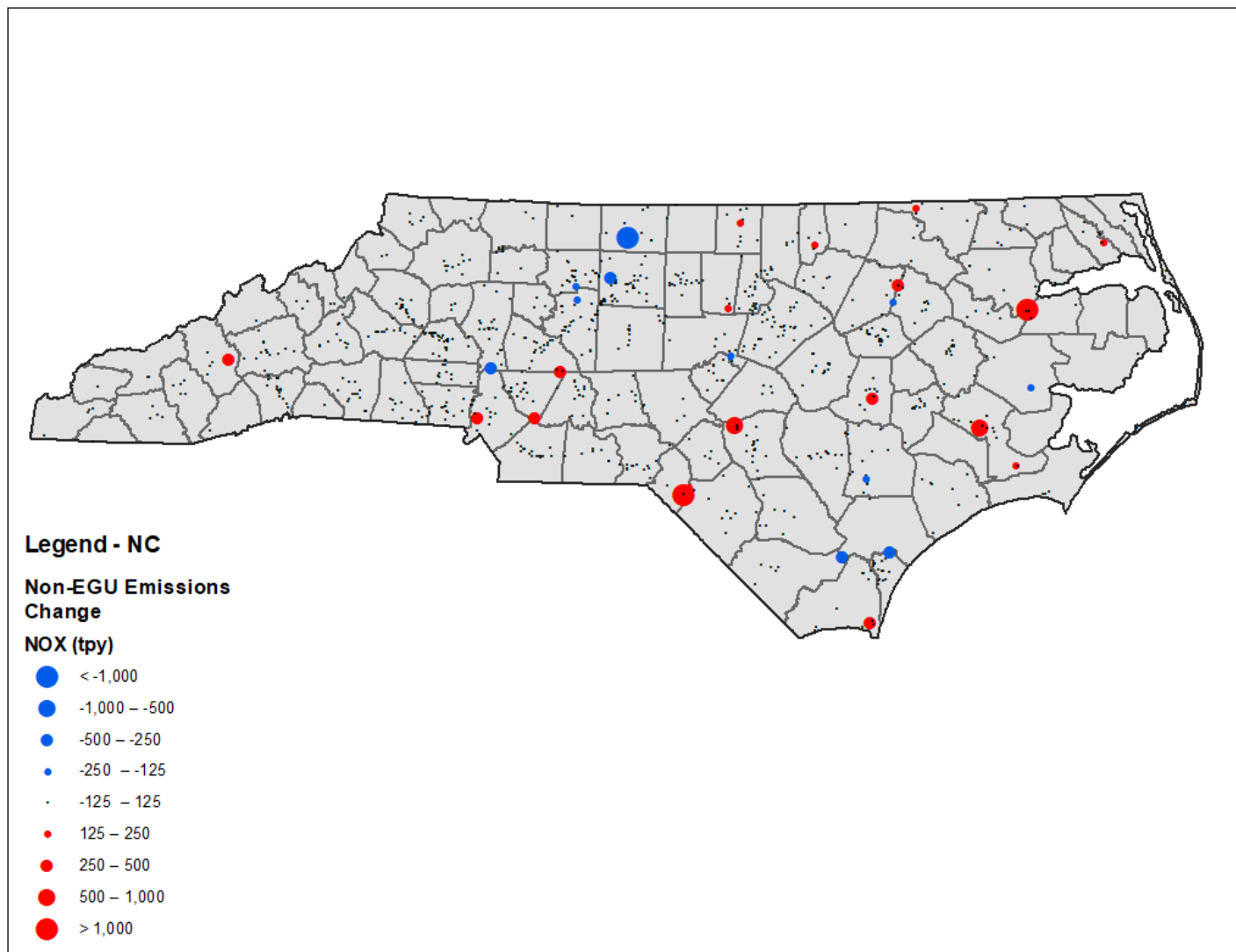
Figure C.6-6. North Carolina Point Non-EGU NO x Emissions Changes from the EPA 2028el Inventory to the Revised 2028 Inventory
