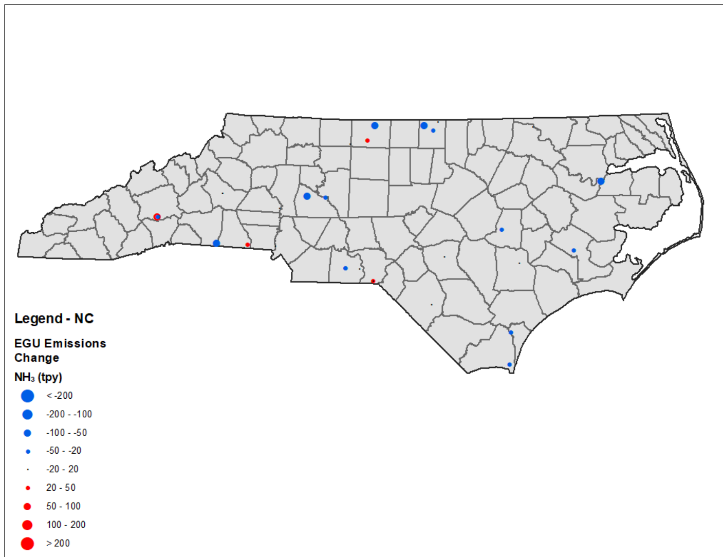
Figure C.6-3. North Carolina Point EGU NH 3 Emissions Changes from the EPA 2028el Inventory to the Revised 2028 Inventory
