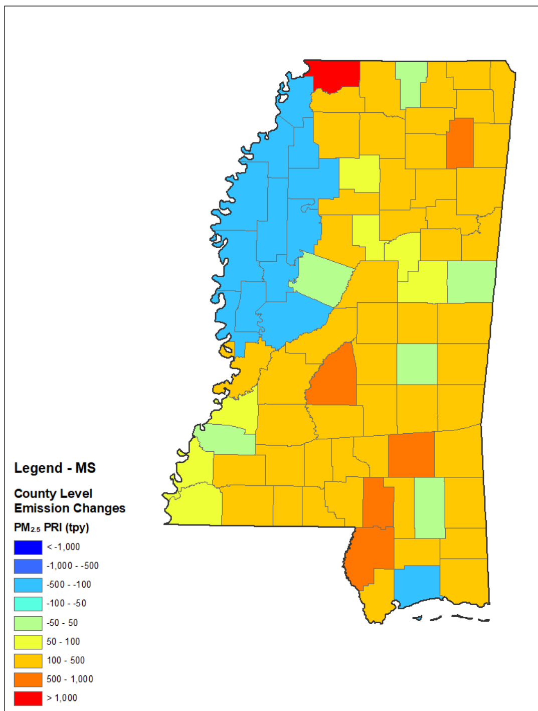
Figure E.5-5. Mississippi County Level PM 2.5 -PRI Emissions Changes from the EPA 2011 Base Year Inventory to the Revised 2028 Inventory (except Biogenic) 72
