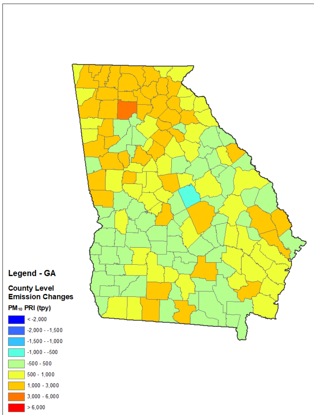
Figure E.3-4. Georgia County Level PM 10 -PRI Emissions Changes from the EPA 2011 Base Year Inventory to the Revised 2028 Inventory (except Biogenic) 67
