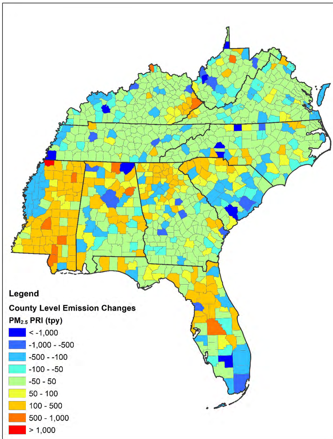
Figure 5-5. County Level PM 2.5 -PRI Emission Changes for the VISTAS Ten States (except Biogenic) 44
