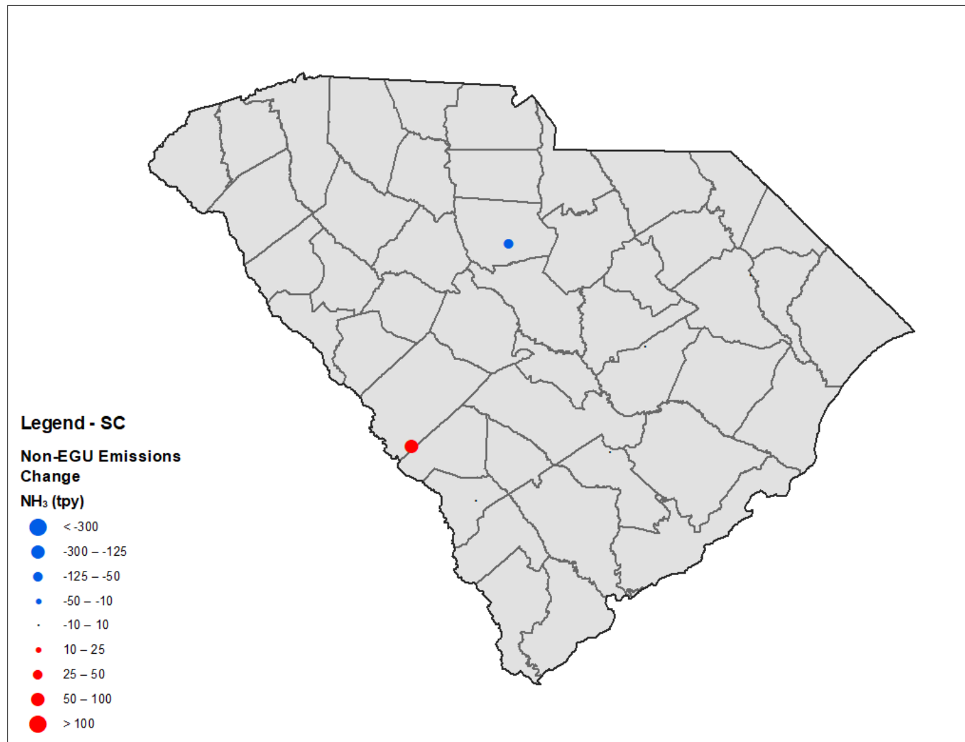
Figure B.7-4. South Carolina Point Non-EGU NH 3 Emissions Changes from the EPA 2028el Inventory to the Revised 2028 Inventory
