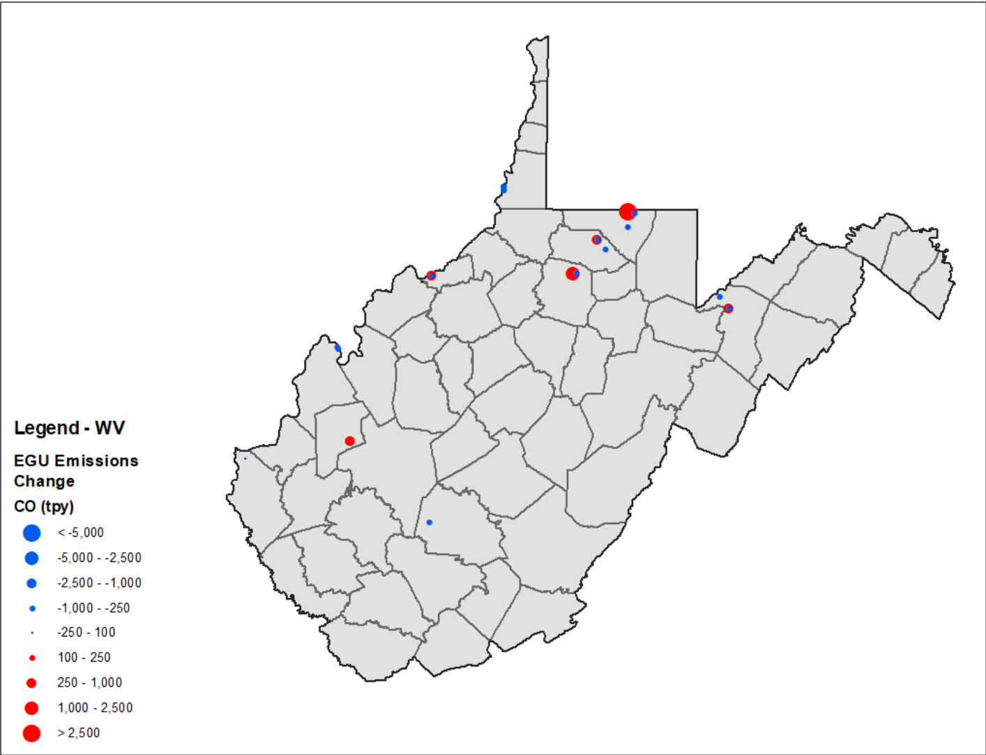
Figure B.10-1. West Virginia Point EGU CO Emissions Changes from the EPA 2028el Inventory to the Revised 2028 Inventory
