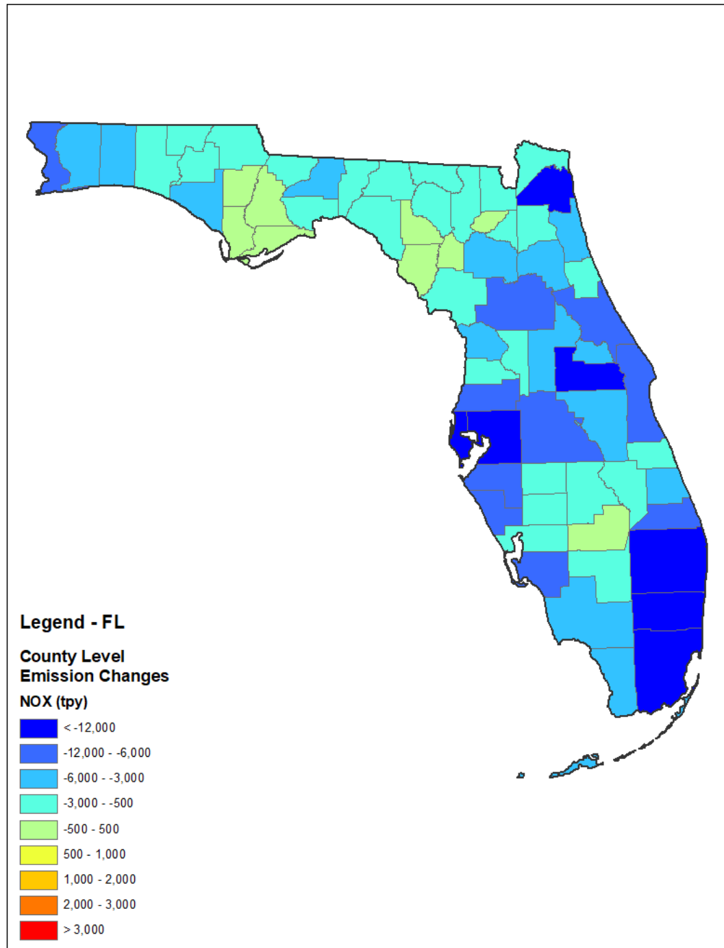
Figure E.2-3. Florida County Level NO x Emissions Changes from the EPA 2011 Base Year Inventory to the Revised 2028 Inventory (except Biogenic)
