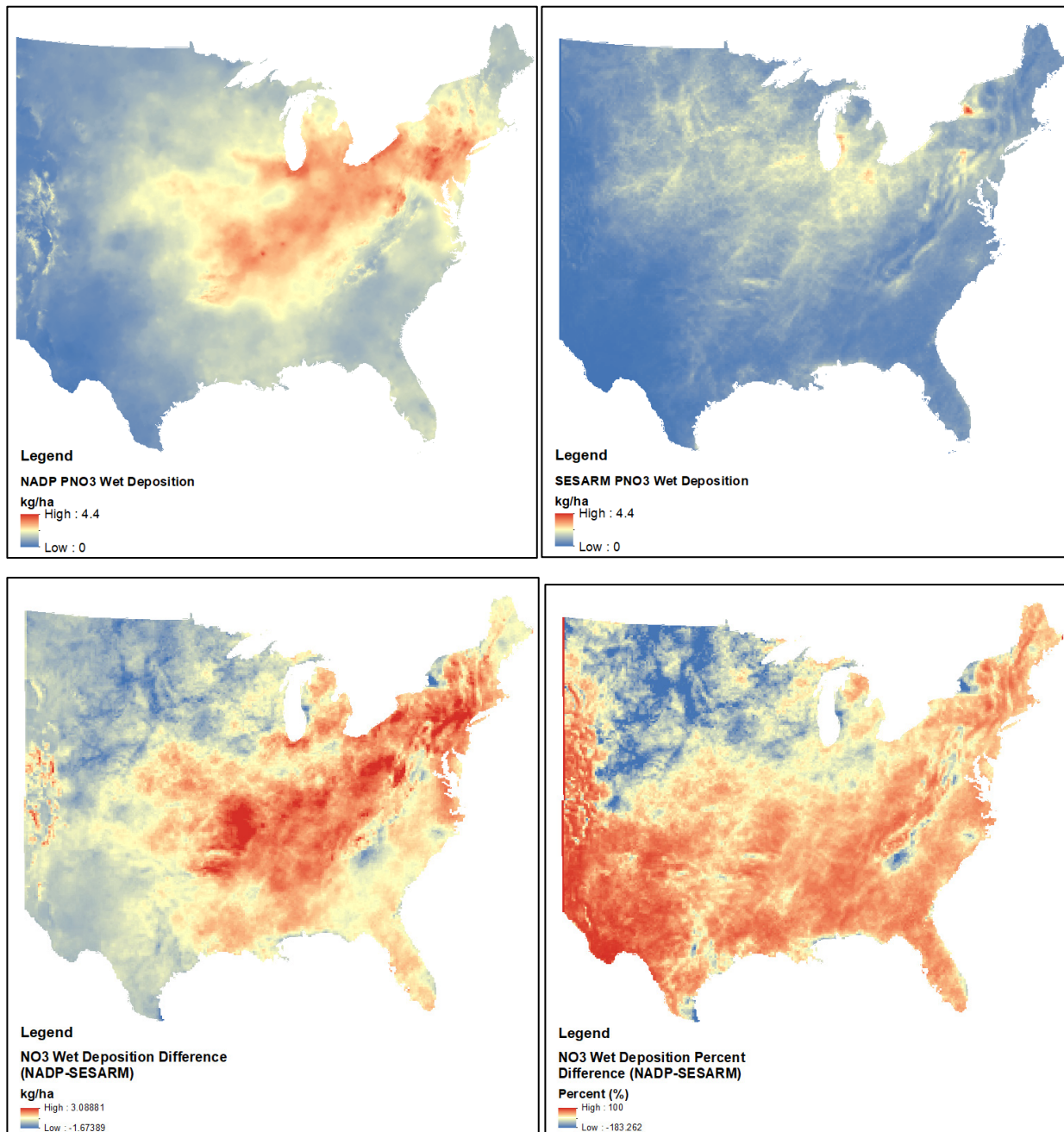
Figure 7-39. Plots of Total Annual Particulate \text{NO}_3^+ Wet Deposition. NADP Wet Deposition (top left), SESARM Wet Deposition (top right), Difference (bottom left), Percent Difference 101 (bottom right).
