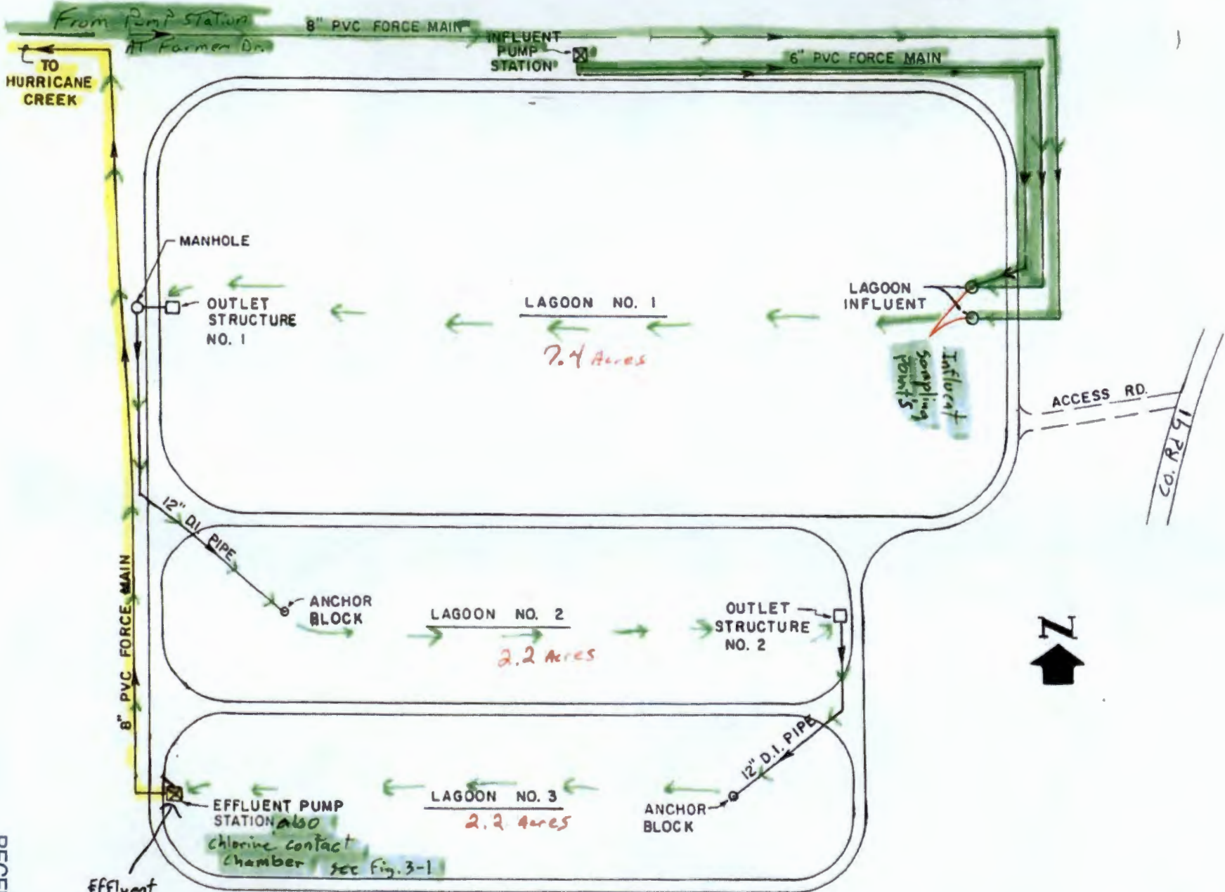
Process Flow Diagram SLOCOMB WASTEWATER TREATMENT PLANT
