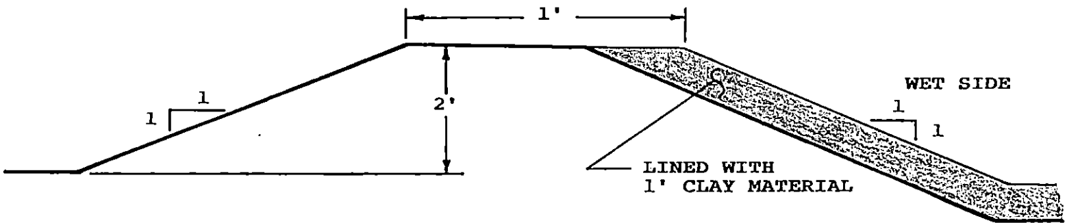
SIDE VIEW
