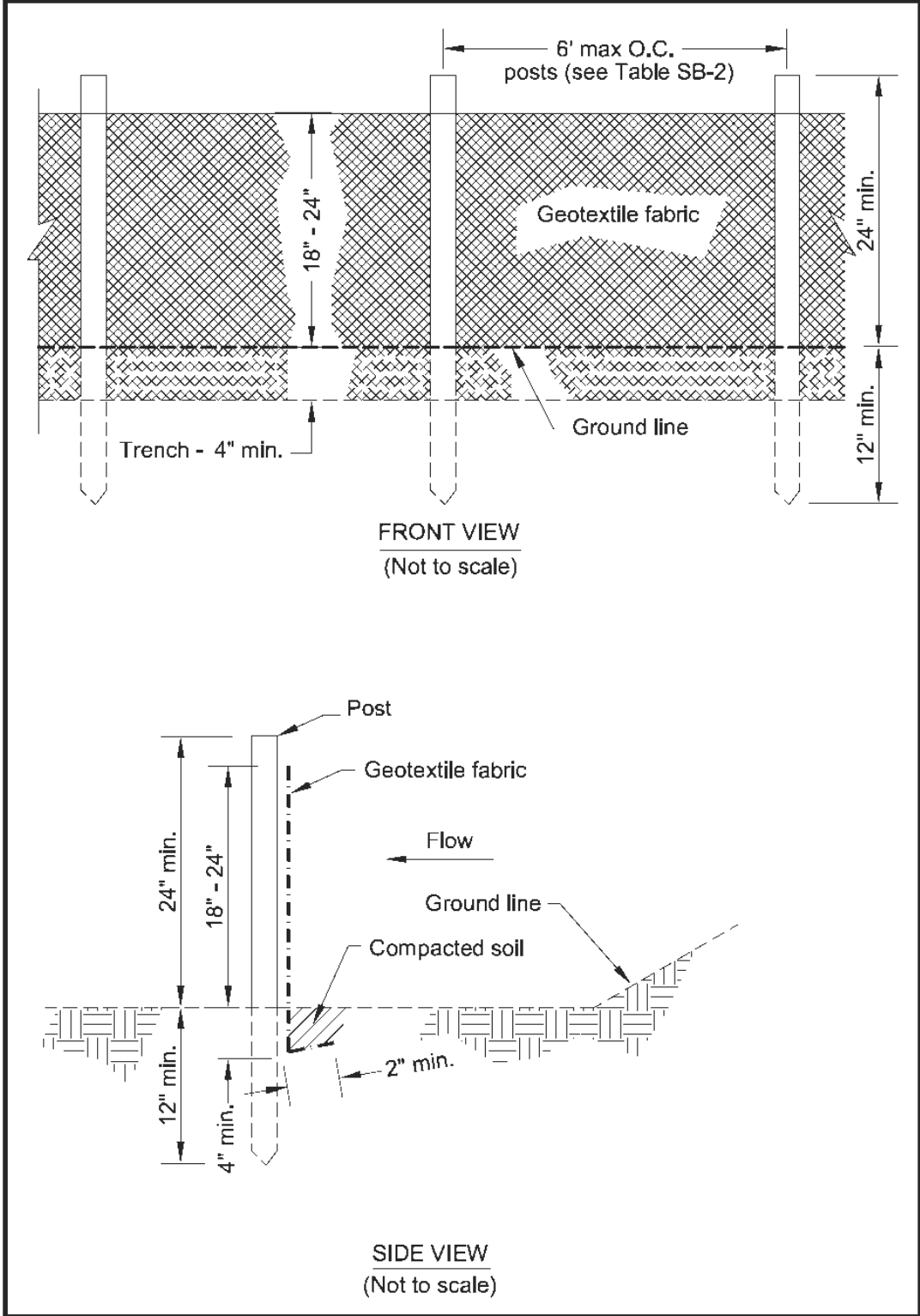
Figure SB-3 Silt Fence – Type C (1) For post material requirements see Tables SB-2 and SB-3
