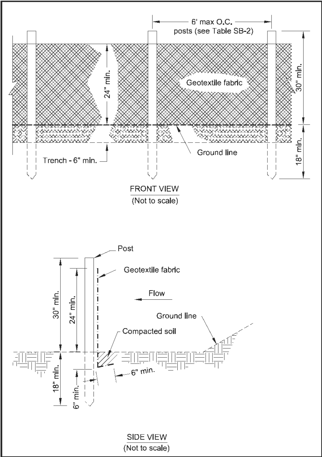
Figure SB-2 Silt Fence - Type B (1) For post material requirements see Tables SB-2 and SB-3
