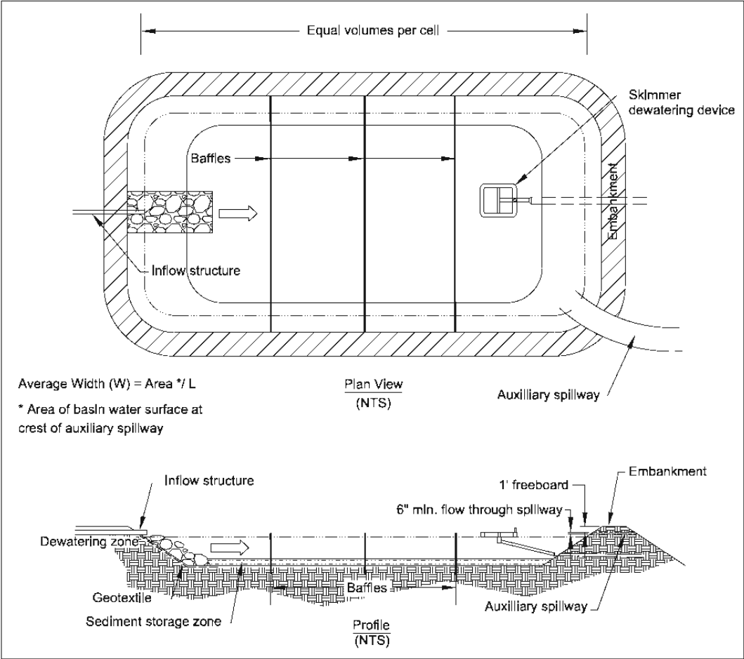
Figure SBN-5 Example of a sediment basin with a skimmer outlet and emergency spillway (modified from Pennsylvania Erosion and Sediment Control Manual, March, 2000)
