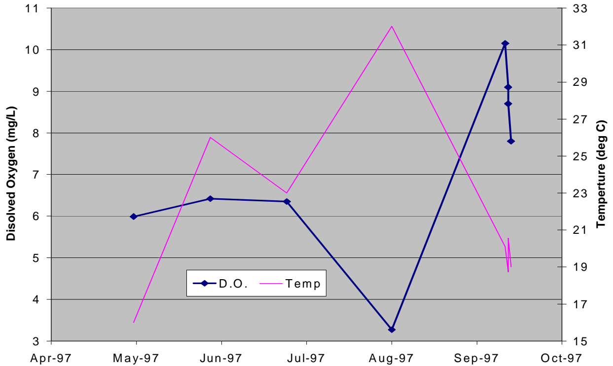
Figure 2.1 Dissolved Oxygen vs. Temperature Data
