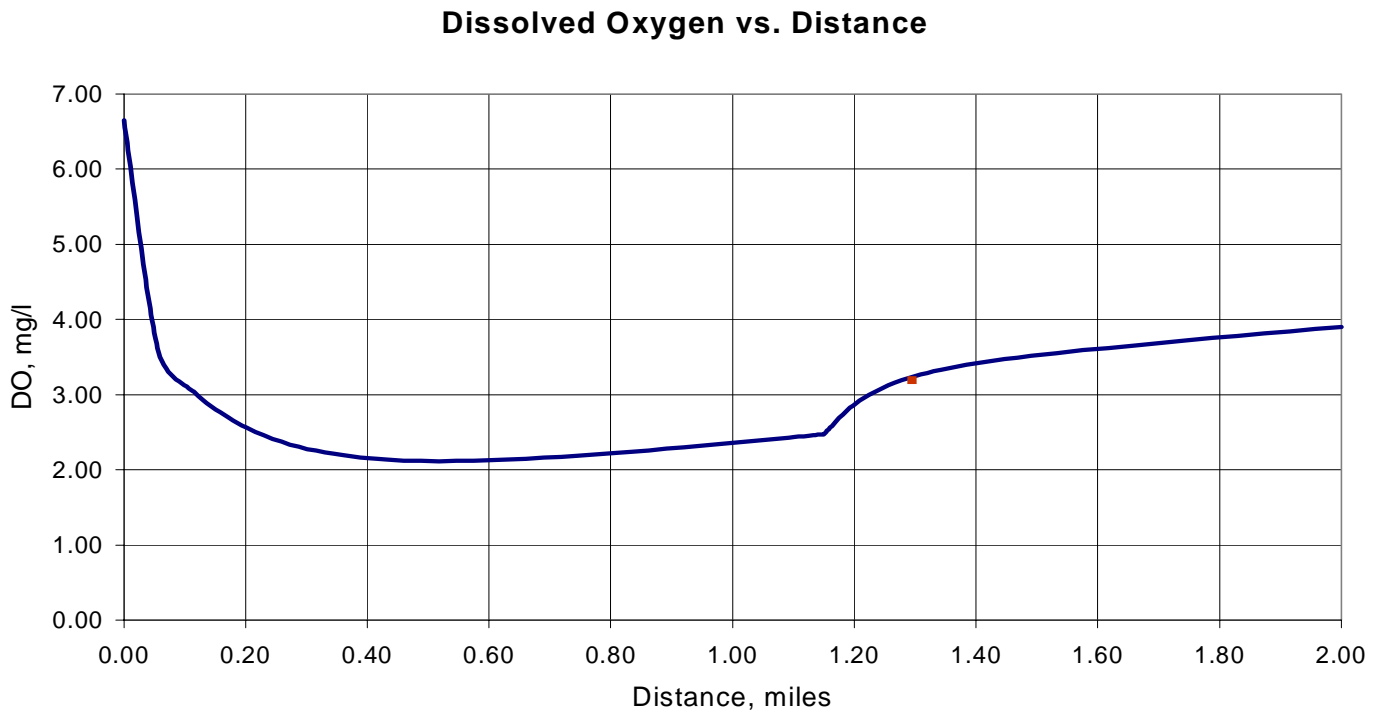
Figure 4-3. Calibrated Model D.O. Predictions vs. Actual D.O. Field Data.
