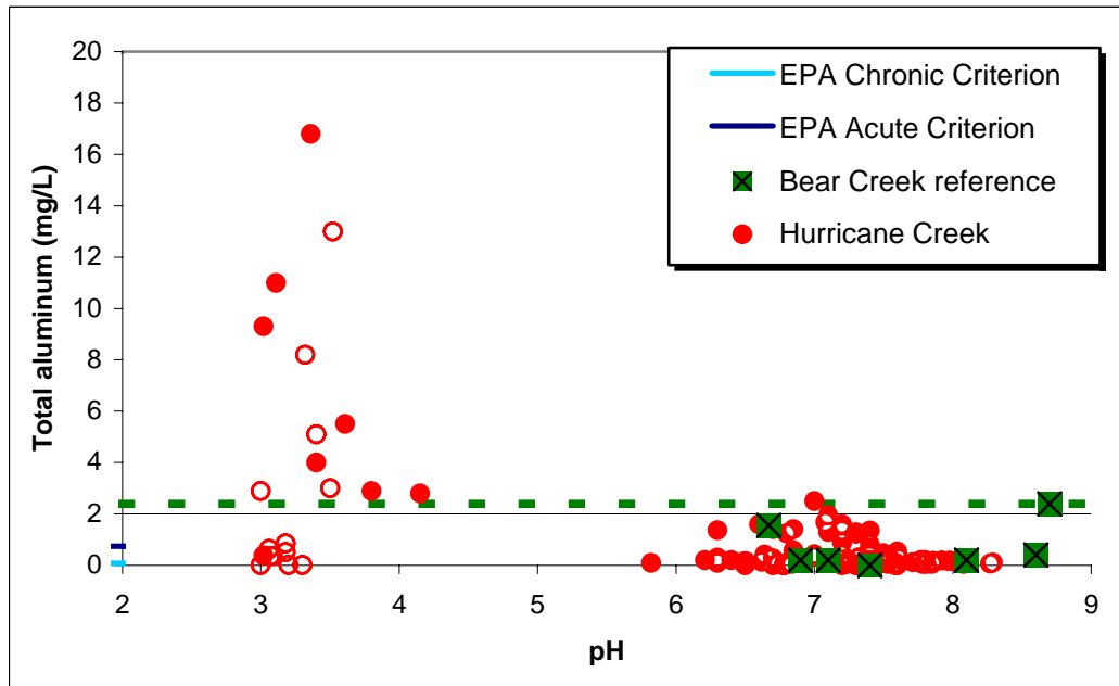
Figure 6. pH and Total Aluminum Concentrations in Hurricane Creek and Bear Creek
