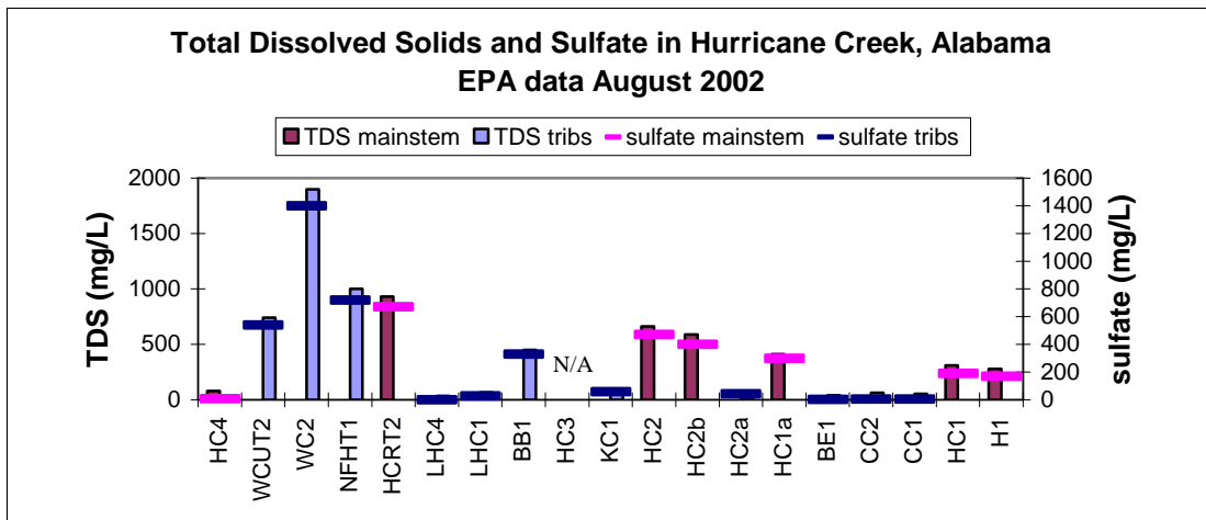
Figure 5. Total Dissolved Solids and Sulfate in Hurricane Creek.
