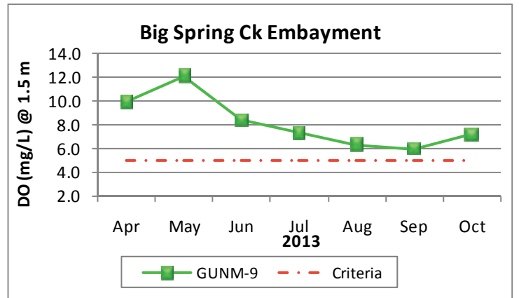
Figure 6. Monthly DO concentrations at 1.5 m (5 ft) for Big Spring Ck embayment station of Guntersville Reservoir collected April-October 2013. ADEM Water Quality Criteria pertaining to reservoir waters require a DO concentration of 5.0 mg/L at this depth.
