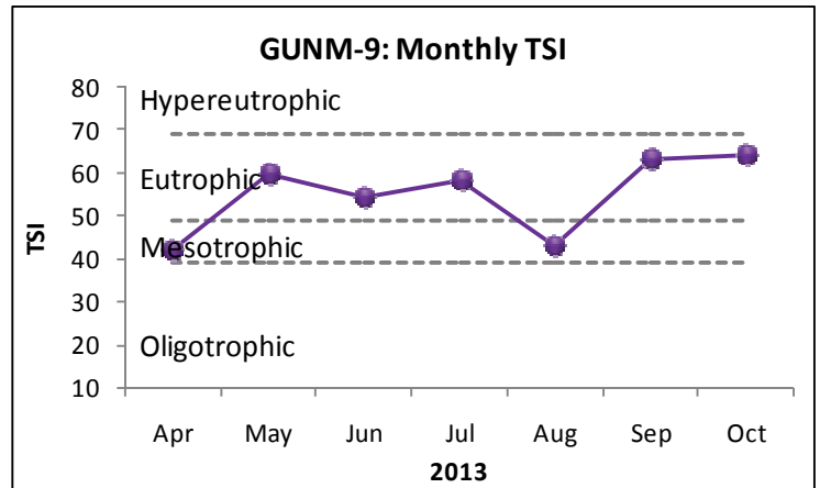
Figure 4. Mean growing season (2003-20013) and monthly (April-October, 2013) TN, TP, chl a and TSI measured in the Big Spring Creek embayment of Guntersville Reservoir. Vertical axis ranges are set to maximum values reservoir-wide for comparability between embayment reports within the same reservoir.
