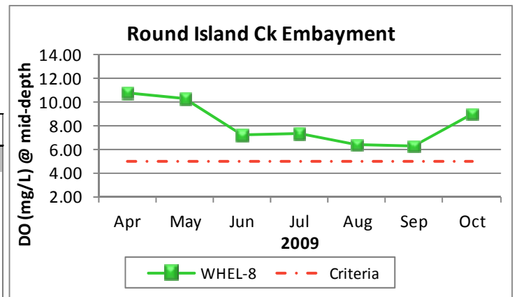
Figure 6. Monthly DO concentrations at mid-depth for Round Island Creek embayment station of Wheeler Reservoir collected April-October 2009. ADEM Water Quality Criteria pertaining to reservoir waters require a DO concentration of 5.0 mg/L at this depth.
