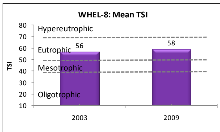
Figure 4. Mean growing season (2003-2009) and monthly (April-October, 2009) TN, TP, chl a and TSI measured in the Round Island Creek embayment of Wheeler Reservoir. Vertical axis ranges are set to maximum values reservoir-wide for comparability between embayment reports within the same reservoir.
