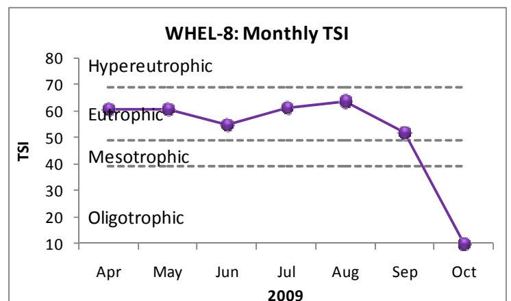
Figure 4. Mean growing season (2003-2009) and monthly (April-October, 2009) TN, TP, chl a and TSI measured in the Round Island Creek embayment of Wheeler Reservoir. Vertical axis ranges are set to maximum values reservoir-wide for comparability between embayment reports within the same reservoir.
