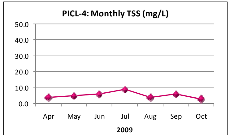
Figure 4. Mean growing season (2003-2009) and monthly (April-October, 2009) chl a , TSI, and TSS measured in the Second Creek embayment of Pickwick Reservoir. Vertical axis ranges are set to maximum values reservoir-wide for comparability between embayment reports within the same reservoir.
