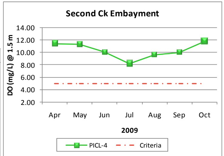
Figure 6. Monthly DO concentrations at 1.5 m (5 ft) for Second Creek embayment station of Pickwick Reservoir collected April-October 2009. ADEM Water Quality Criteria pertaining to reservoir waters require a DO concentration of 5.0 mg/L at this depth .
