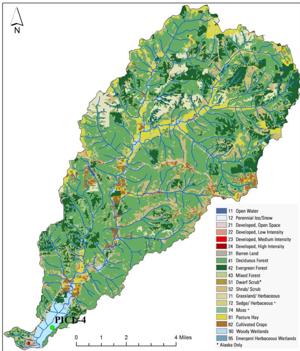
Figure 3. Land use within the Second Creek watershed at PICL-4.
