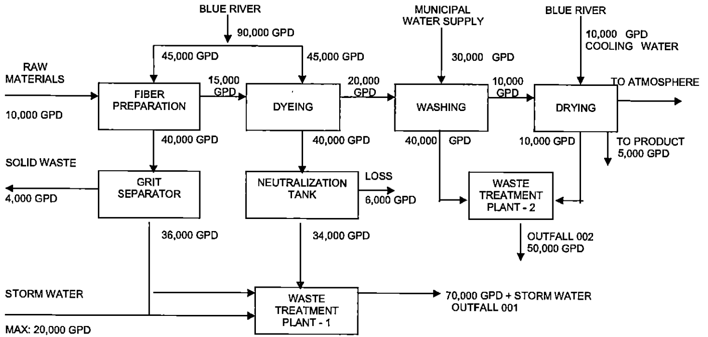
SCHMATIC OF WATER FLOW BROWN MILLS INC CITY, COUNTY, STATE
