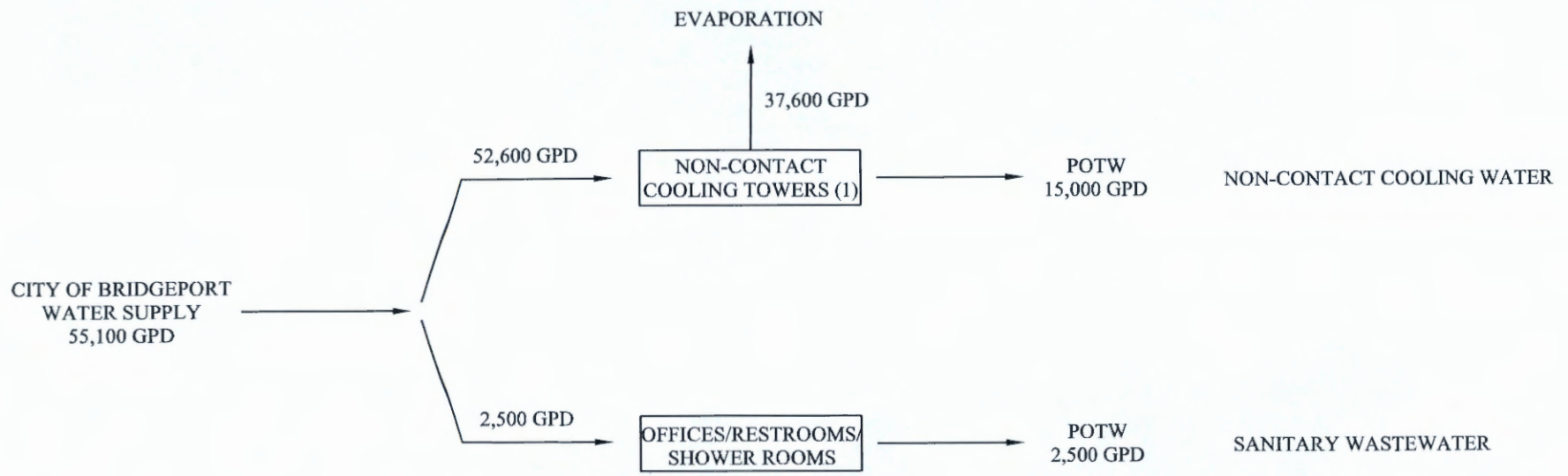
FIGURE 3 TENNESSEE ALLOYS COMPANY WATER FLOW SCHEMATIC
