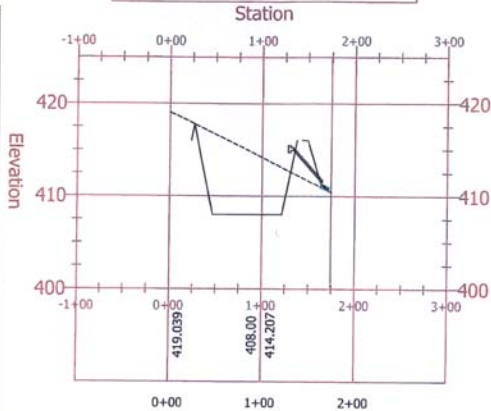
BASIN 001 ALIGNMENT PROFILE
