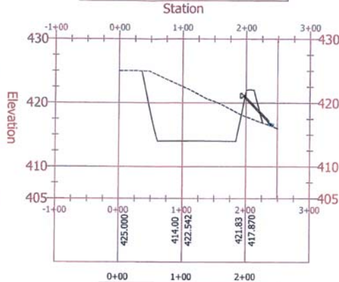
Basin 4 Alignment PROFILE
