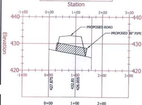
HAUL ROAD PIPE PROFILE
