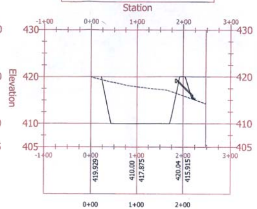
BASIN 003 ALIGNMENT PROFILE
