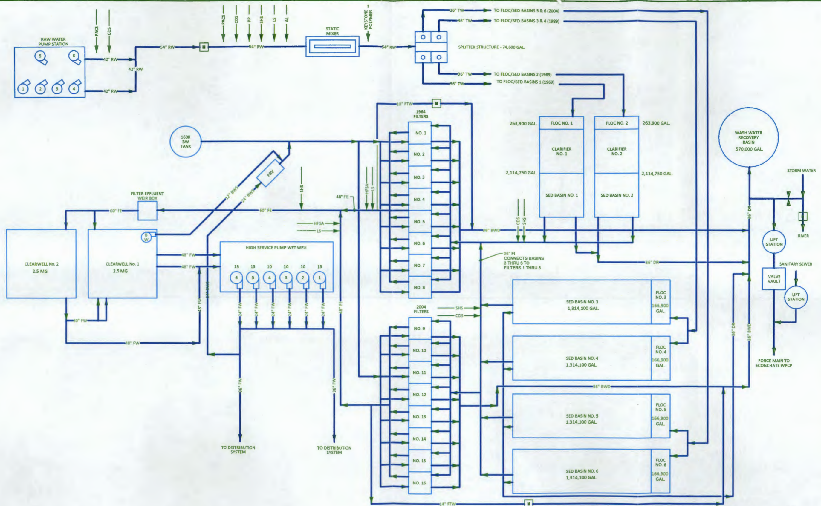
FIGURE 2-4 MONTGOMERY COMP PLAN UPDATE CT PERRY WTP PROCESS FLOW DIAGRAM
